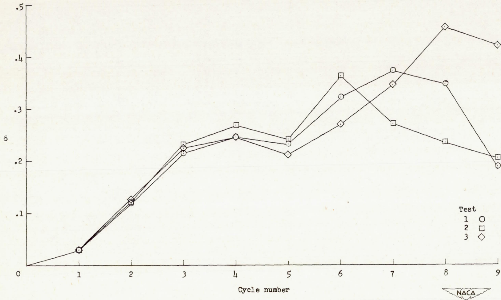
(c) Variation of \delta for large beam-tank system.
