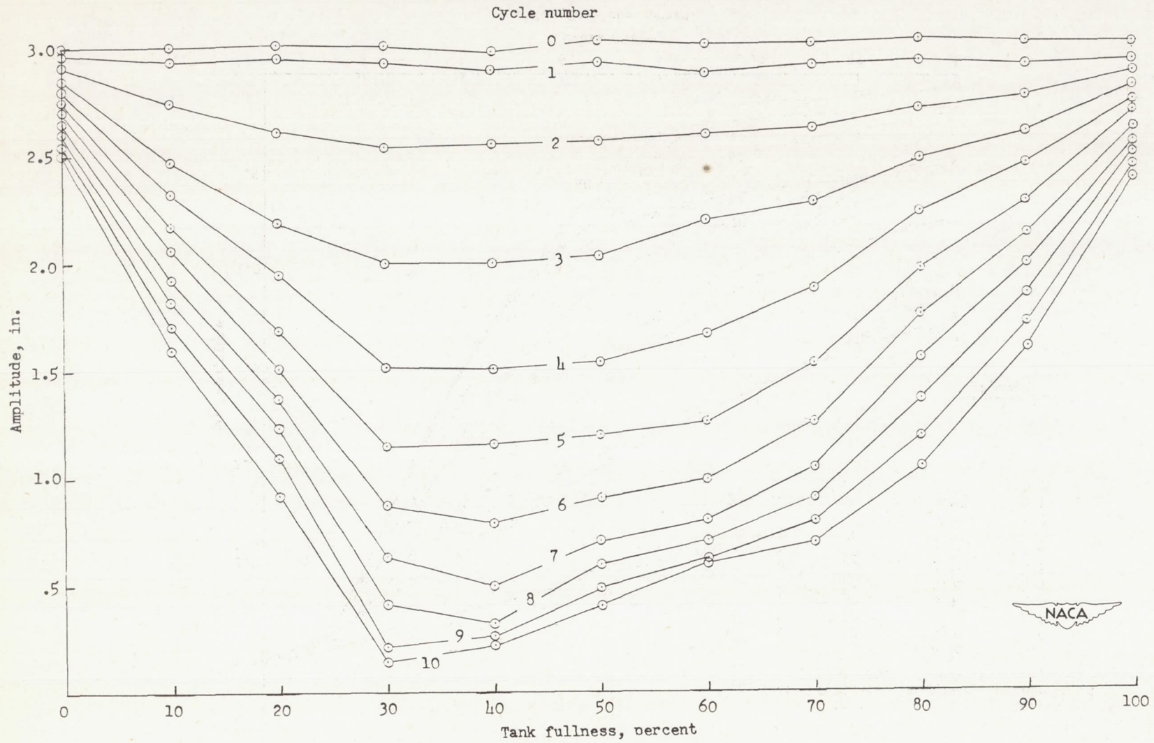
(b) Cross-plot of envelope curves.
