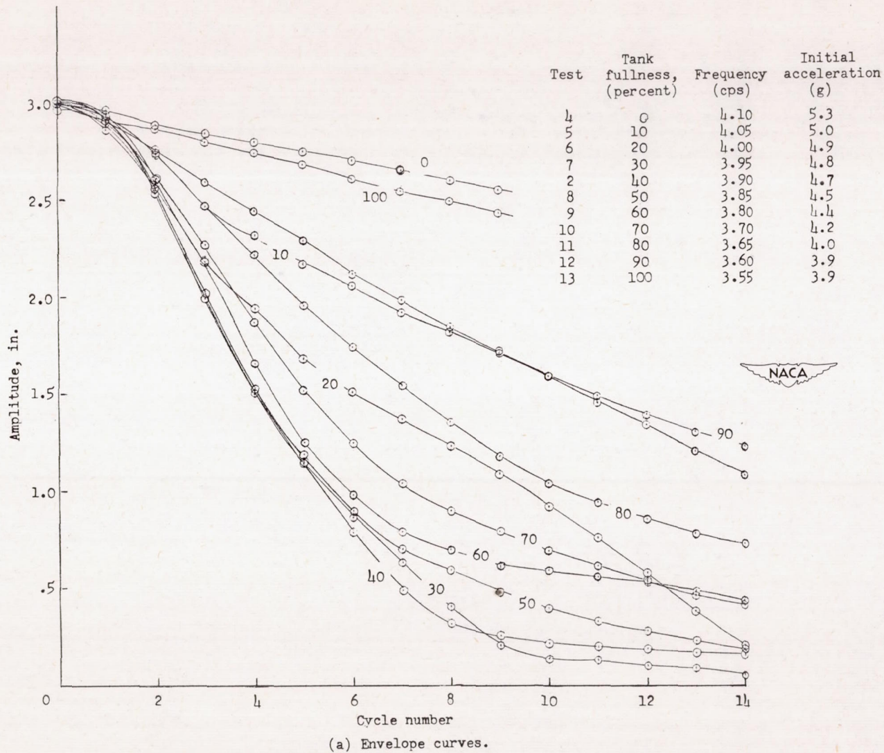
Figure 8.- Effects of tank fullness on damping.
