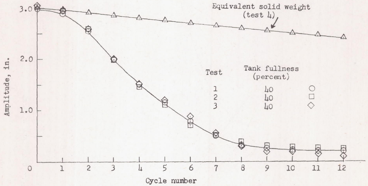
(a) Envelope curves for partly filled tank and equivalent solid weight.
