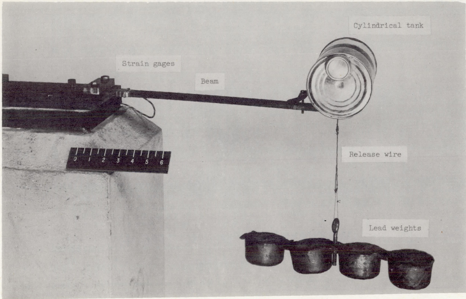
Figure 4.- Small beam-tank system.
