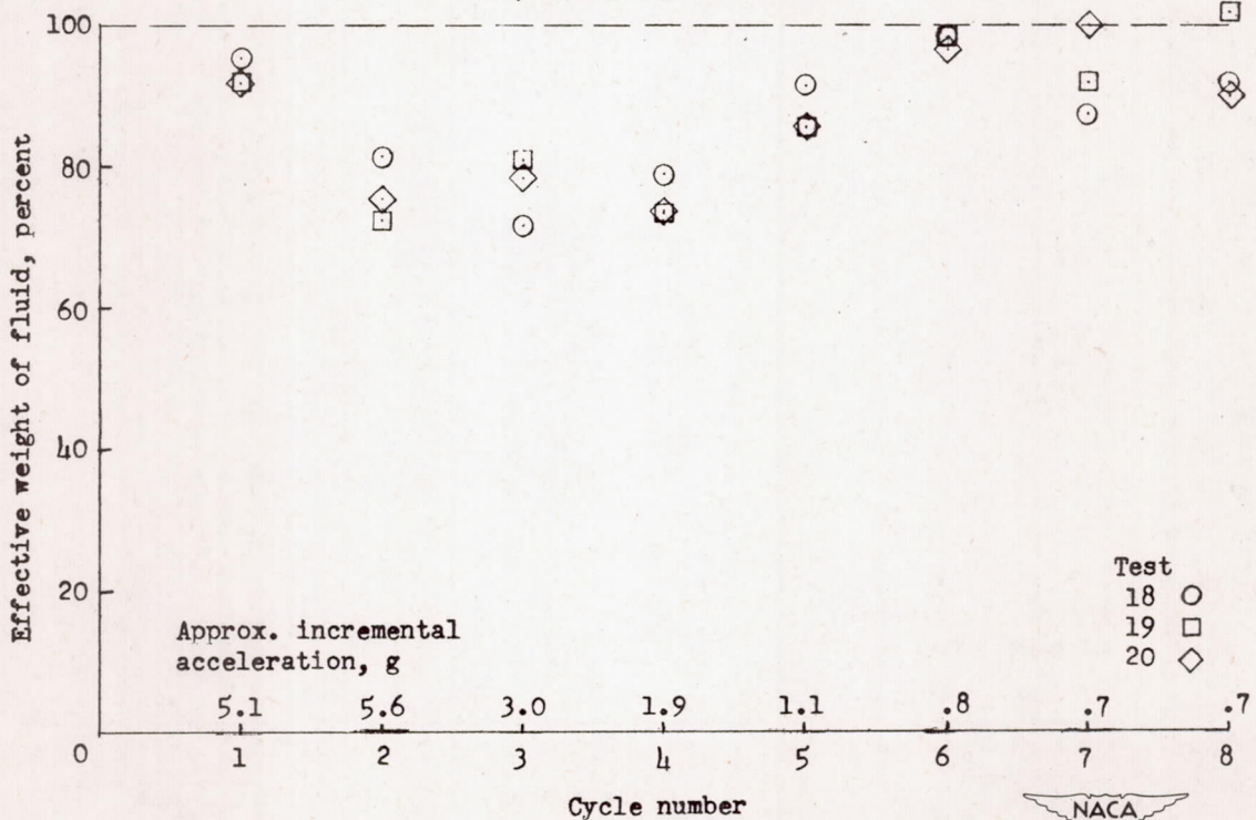
(f) Tank 60 percent full.
