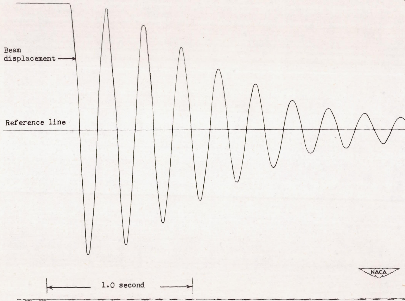
Figure 2.- Typical record for large beam-tank system. Test 2; tank 40 percent full.
