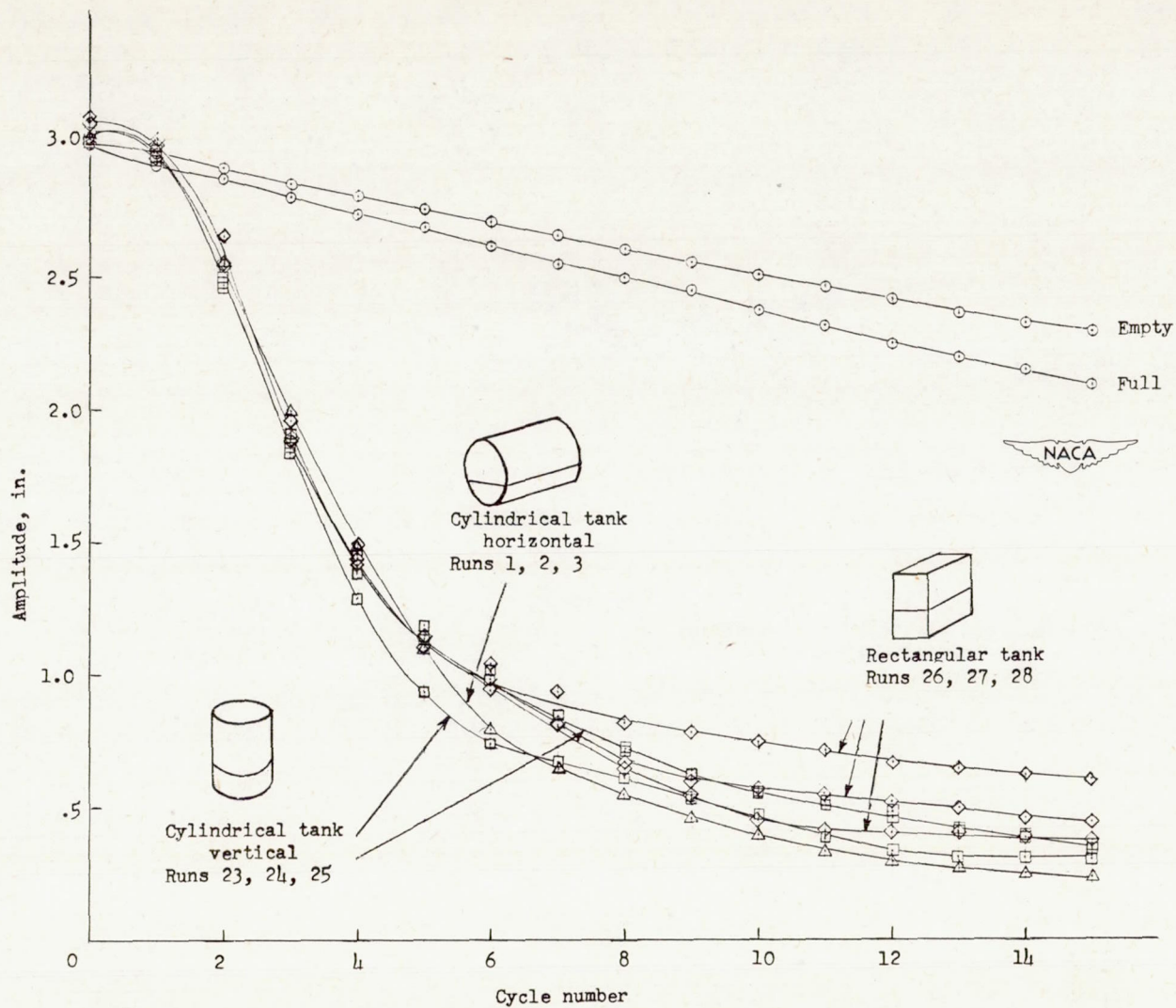
Figure 10.- Effects of tank shape. Large beam-tank system. (All tanks 40 percent full except as noted.)
