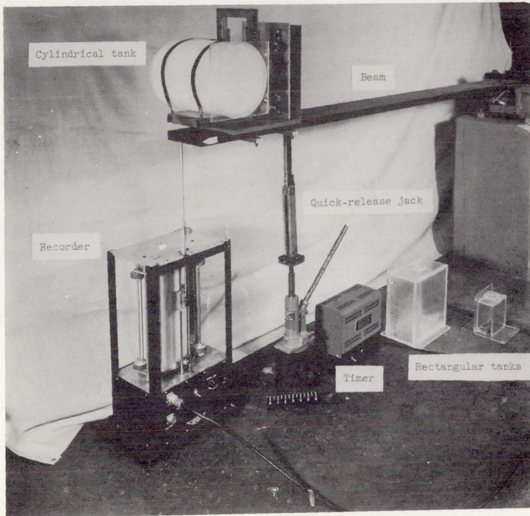
Figure 1.- Large beam-tank system.
