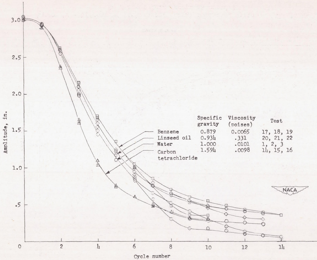
Figure 9.- Effects of fluid viscosity and density.
