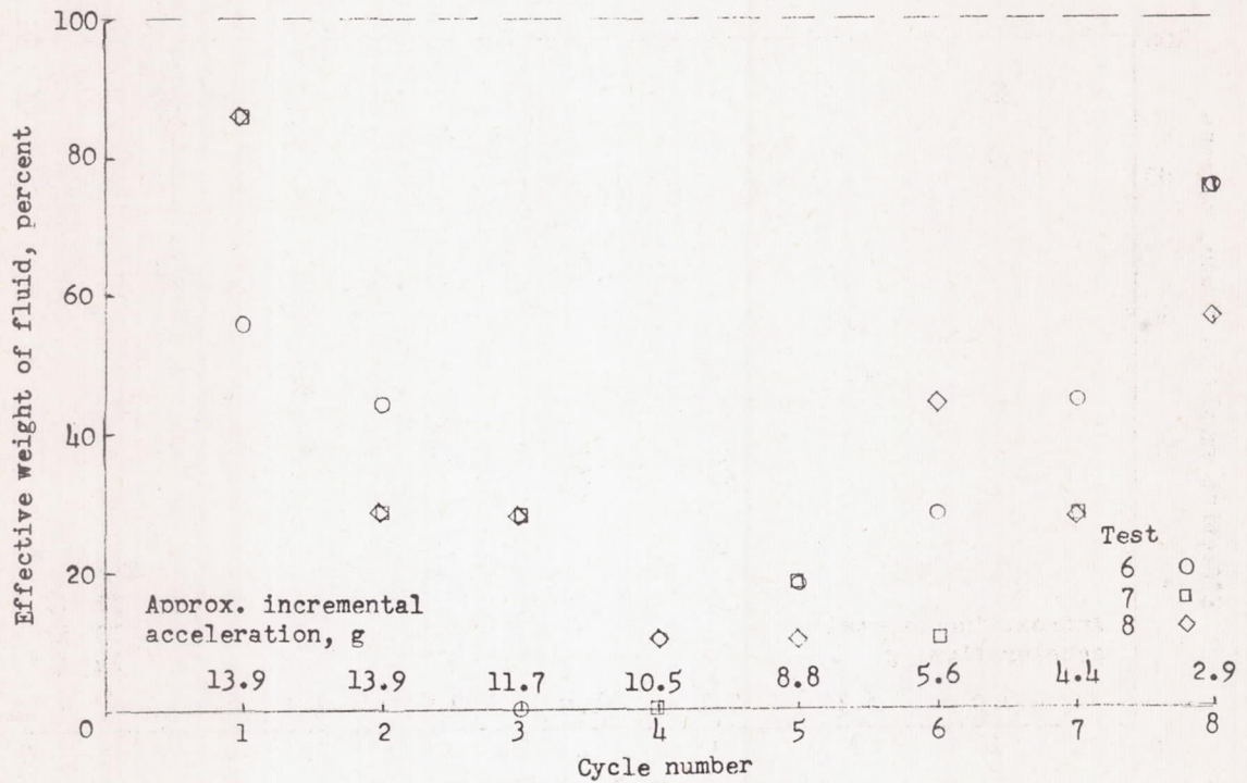
(a) Tank 10 percent full.
