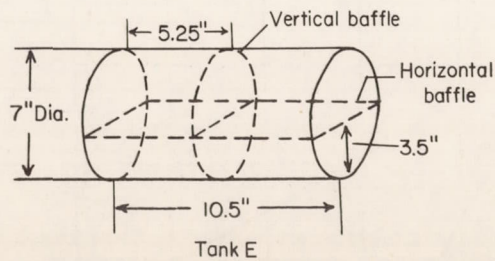
(b) Circular-cylinder tank. Fineness ratio, 1.5.
