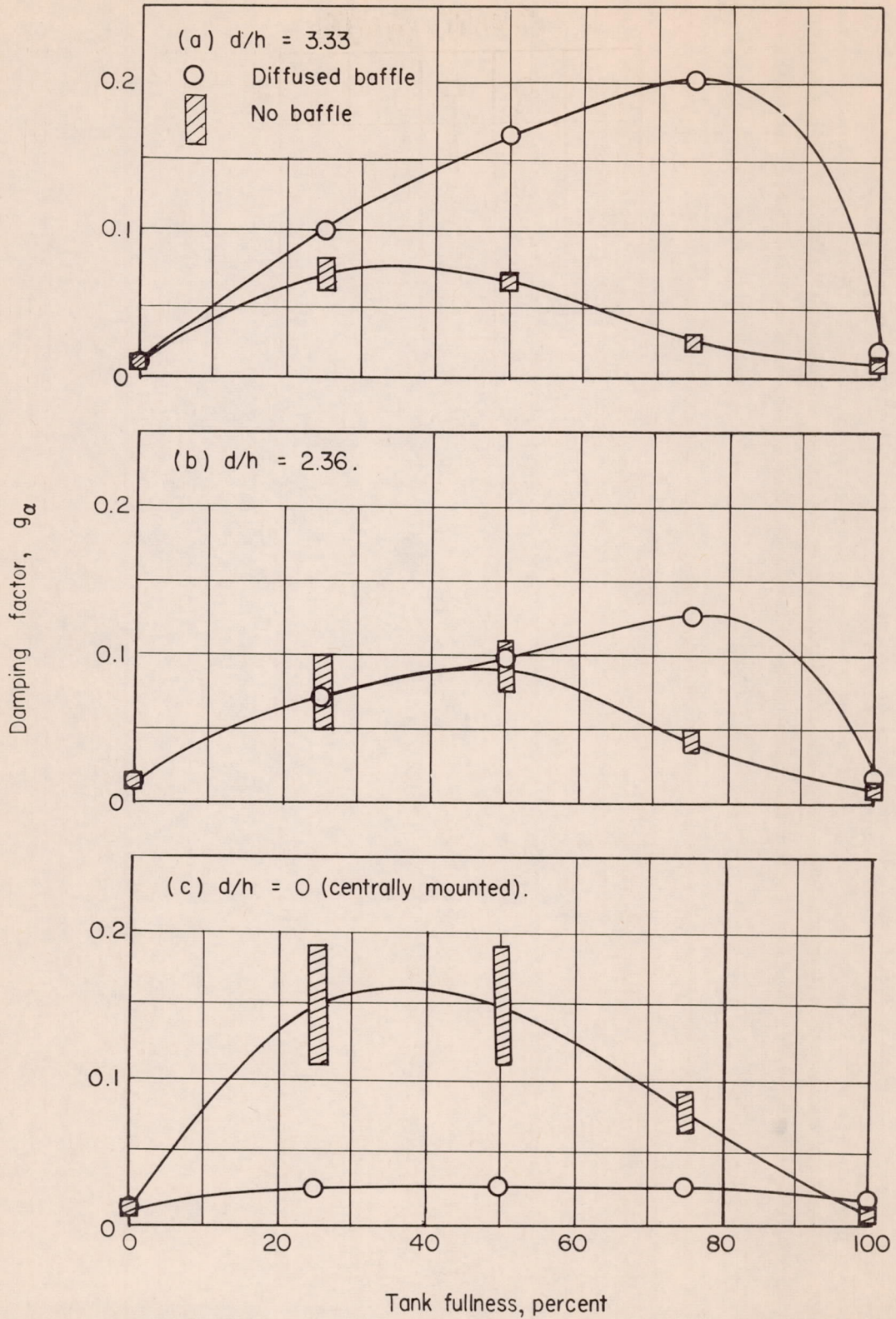
Figure 9.- Effect of diffused baffle on damping factor for tank G.
