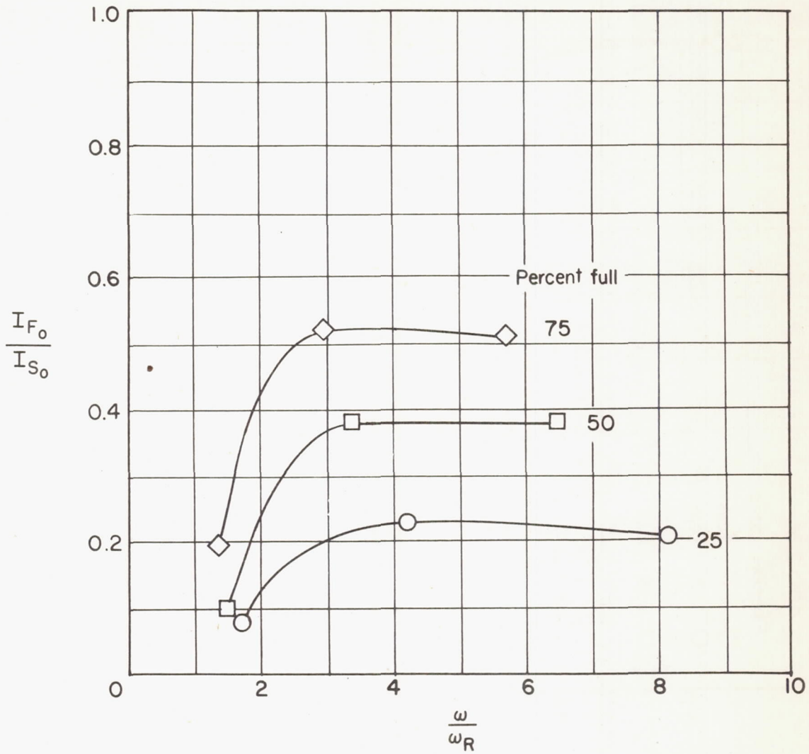
Figure 4.- Effect of frequency on inertia ratio for pylon-mounted tank A. d/h = 3.33 .
