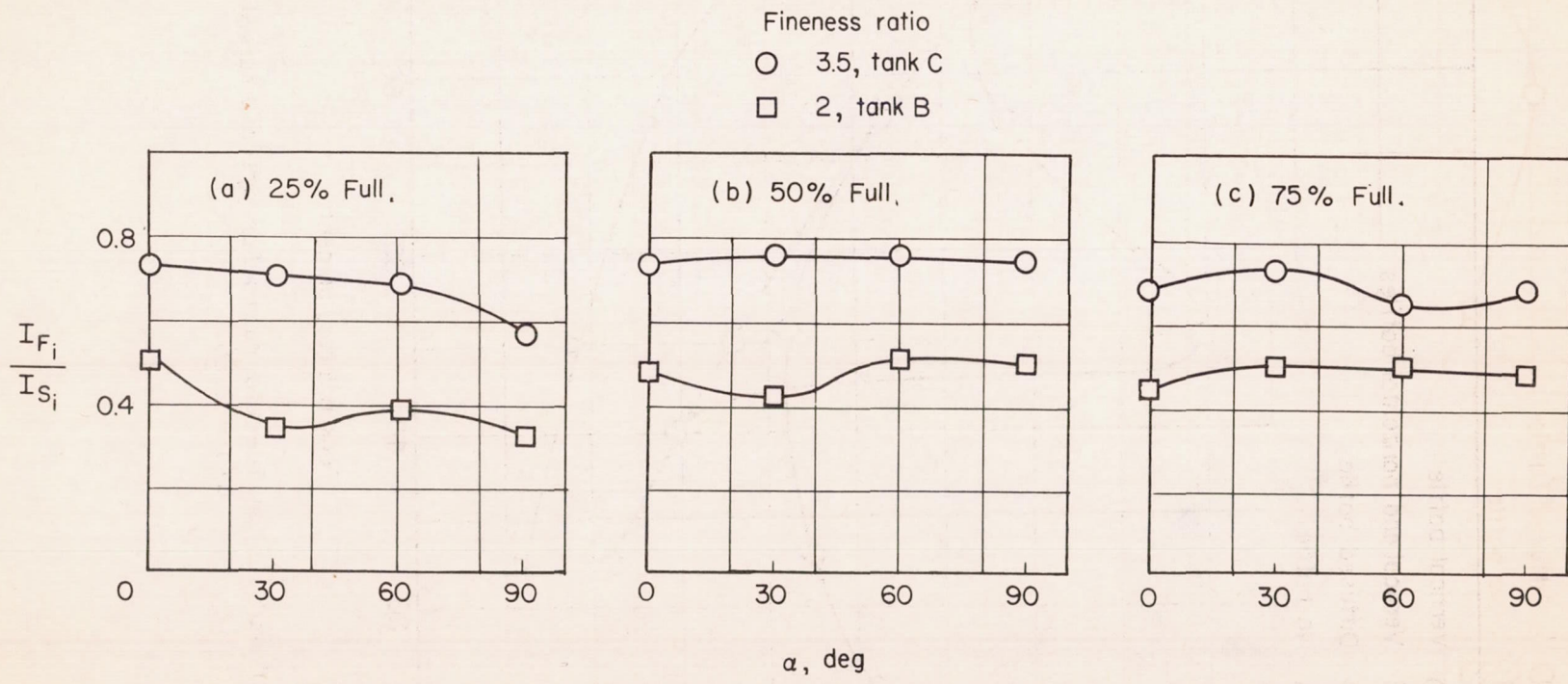
Figure 8.- Effect of angle of attack on inertia ratio for centrally mounted tanks.
