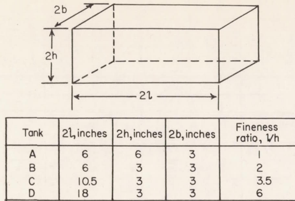
(a) Rectangular tanks.
